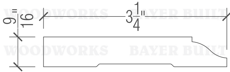
229A BASE
