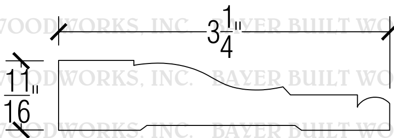
178C CASING
