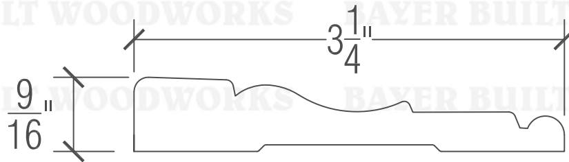
178A CASING
