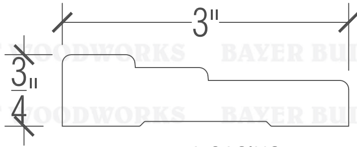
177A CASING
