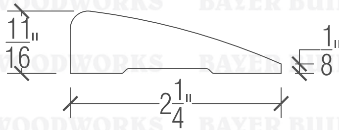
128A CASING
