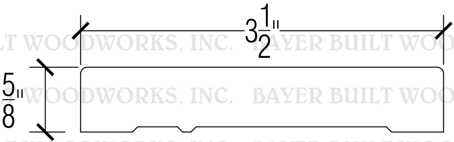
154A CASING
