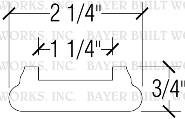
6045 SHOE RAIL
